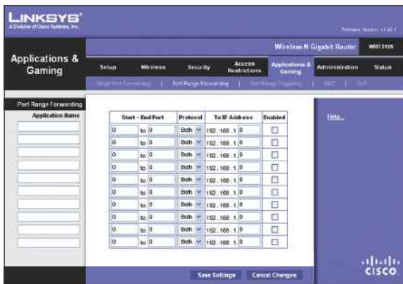
Applications and Gaming &gt; Port Range Forwarding
