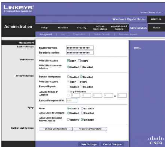
Administration > Management
