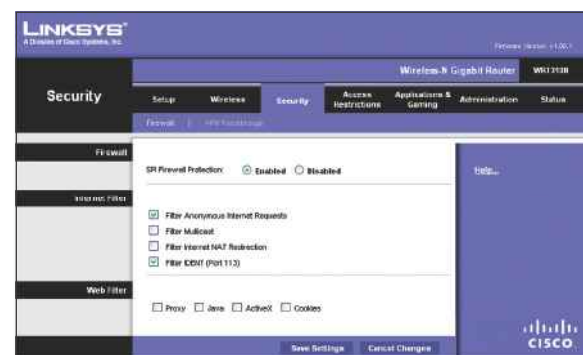
Security > Firewall
