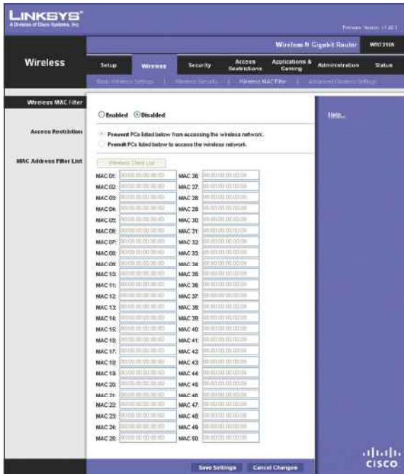
Wireless > Wireless MAC Filter
