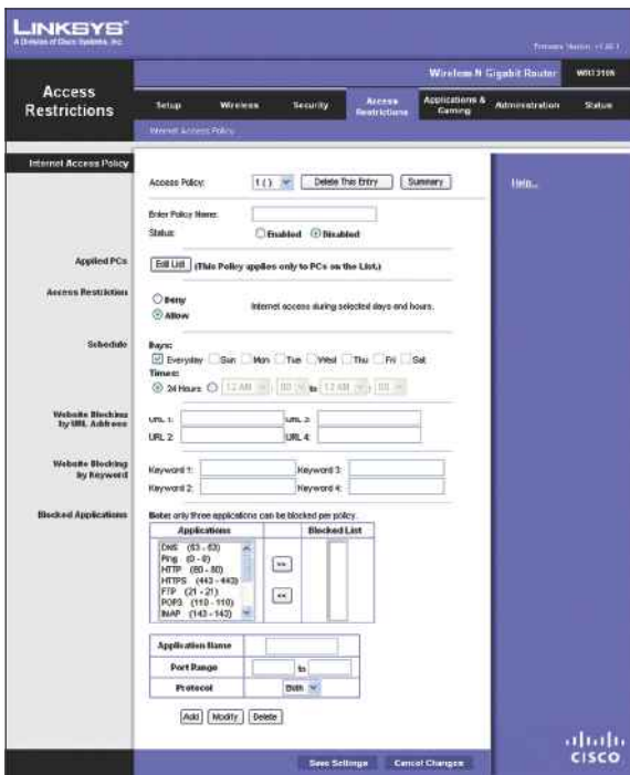
Access Restrictions > Internet Access
