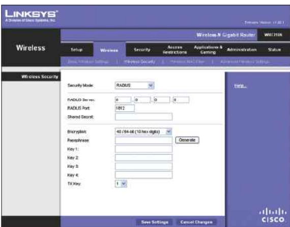
Security Mode > RADIUS
