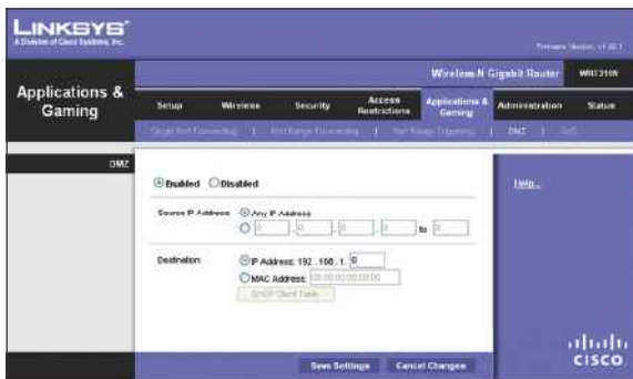
Applications and Gaming &gt; DMZ
