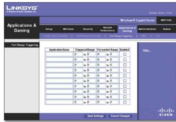
Applications and Gaming &gt; Port Range Triggering
