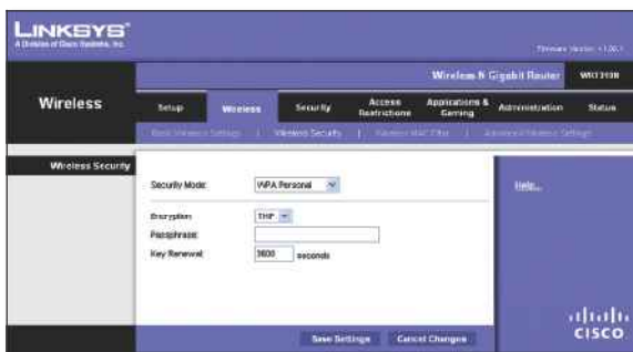
Security Mode > WPA Personal
