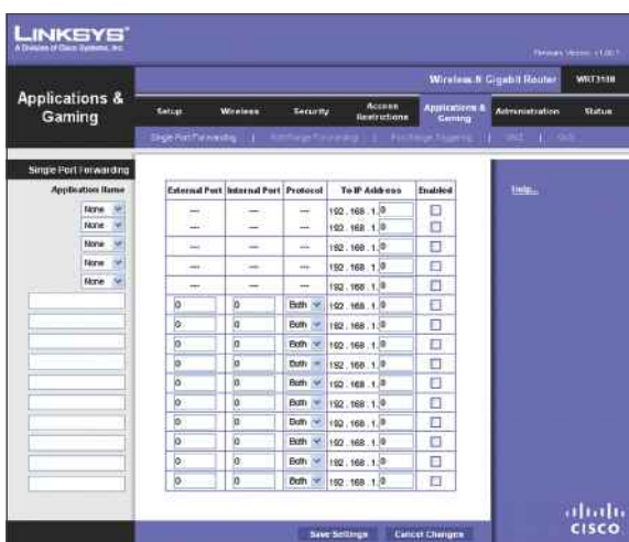
Applications and Gaming > Single Port Forwarding
