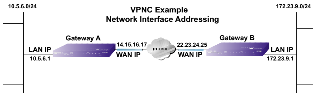
Figure B-4: VPNC Example Network Interface Addressing
